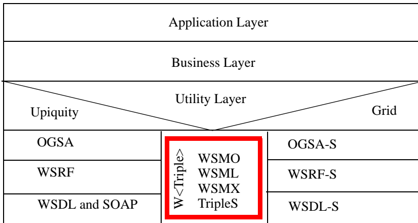
Fig. 1 Semantically empowered service-oriented architectures (SESA).
